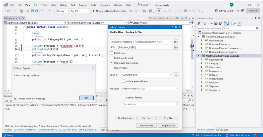
Figure 12.3: Find and replace all matches using regular expressions in Visual Studio
