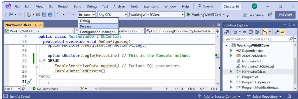
Figure 10.6: Including SQL parameters in logging for debug configuration
