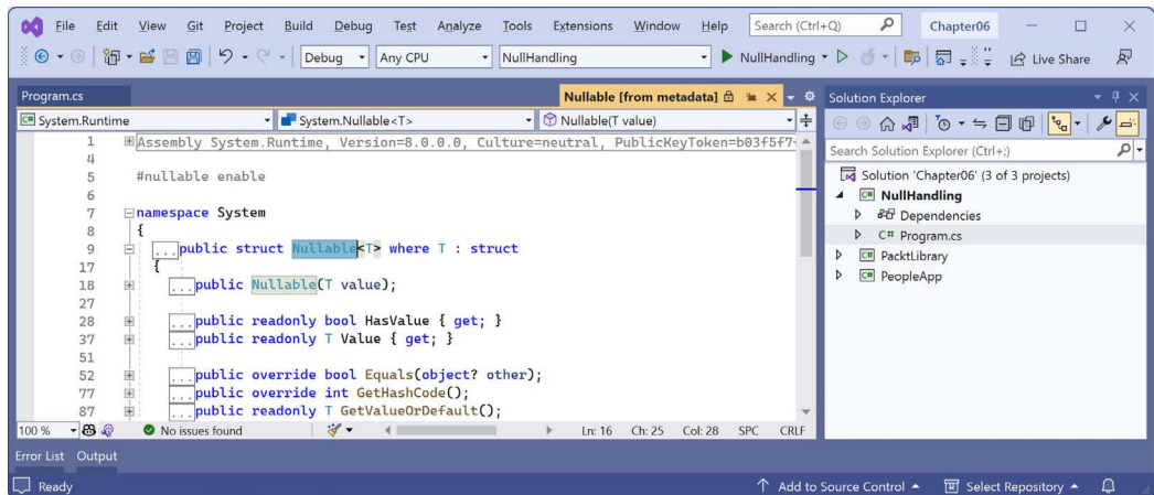
Figure 6.1: Revealing Nullable<T> members
