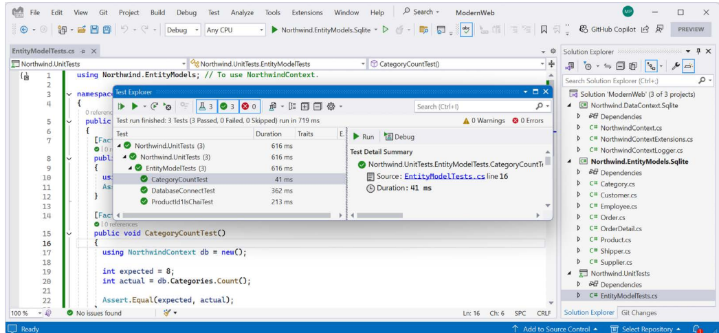
Figure 12.4: Three successful unit tests ran
