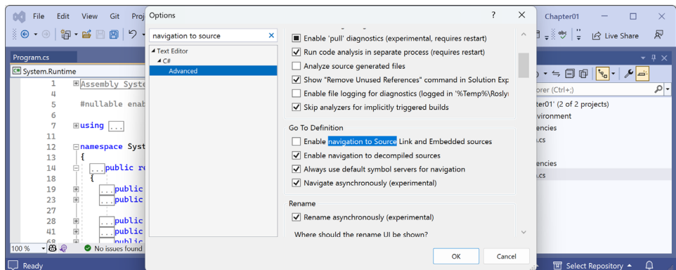
Figure 1.11: Disabling Source Link for the Go To Definition feature
