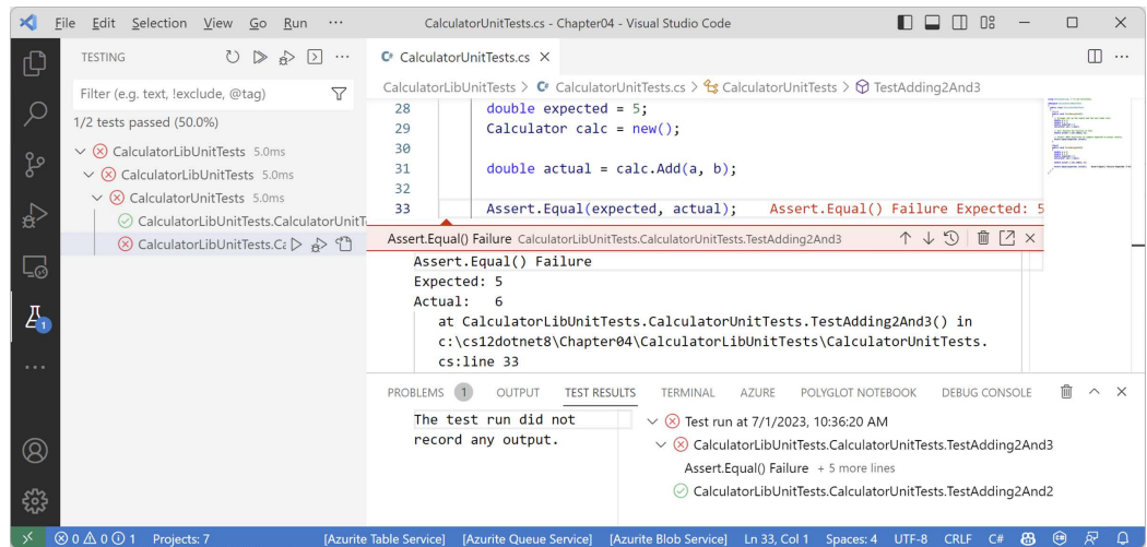
Figure 4.17: The unit test results in VS Code's TEST RESULTS
