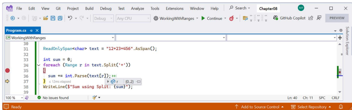
Figure 8.6: A span and range used to split a string efficiently
