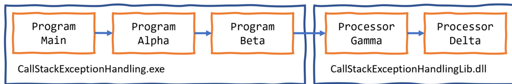
Figure 4.18: A chain of method calls that create a call stack
