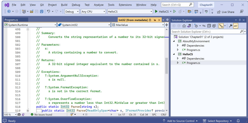
Figure 1.12: The comments for the Parse method with a single string parameter
