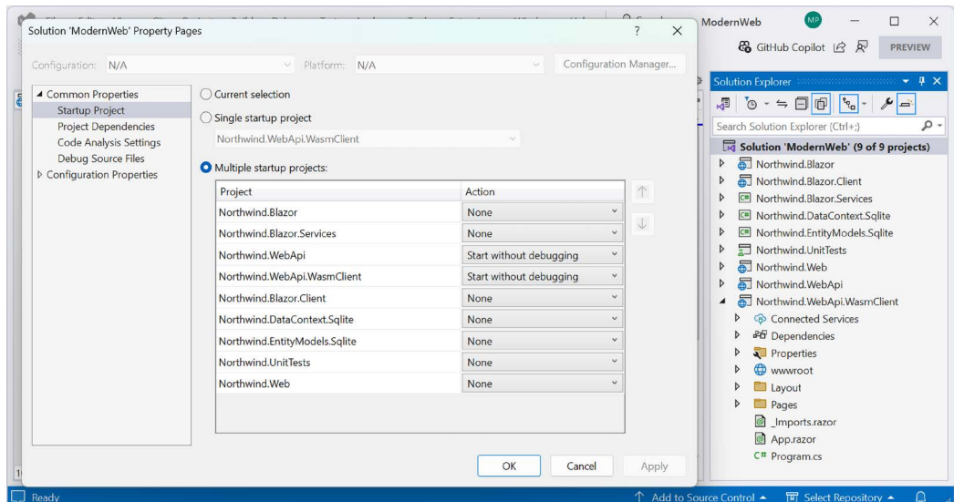
Figure 15.6: Selecting multiple projects to start up in Visual Studio
