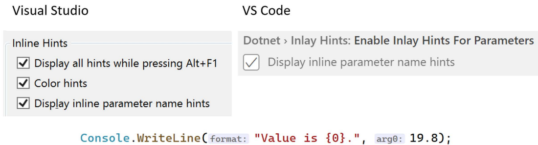
Figure 1.13: Configuring inline hints, aka inlay hints
