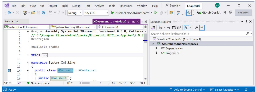
Figure 7.1: Assembly and namespace that contains the XDocument type
