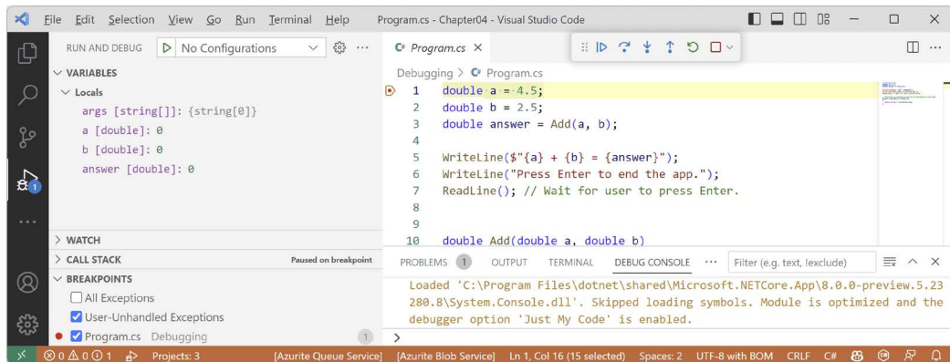
Figure 4.6: Break mode in VS Code
