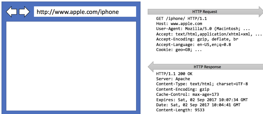
Figure 12.5: An HTTP request and response
