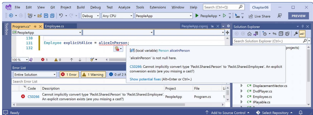
Figure 6.4: A missing explicit cast compile error
