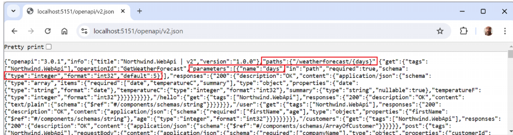
Figure 15.5: OpenAPI JSON documentation for the Northwind web service
