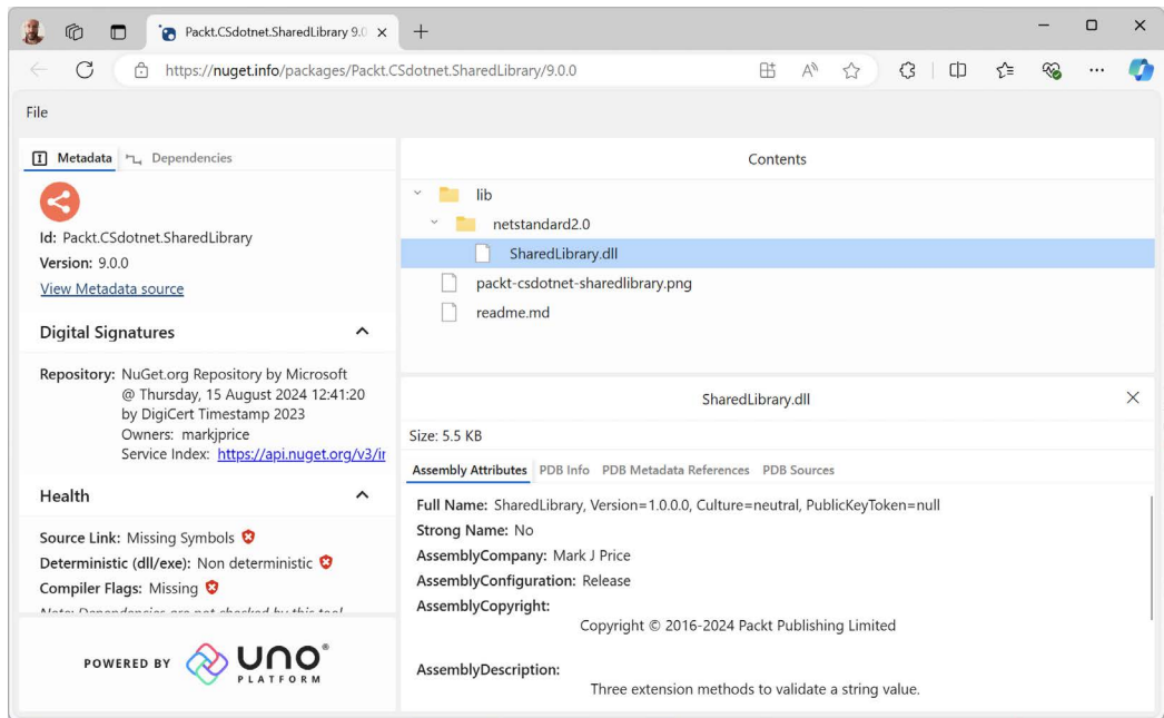
Figure 7.6: Exploring my package using NuGet Package Explorer from Uno Platform
