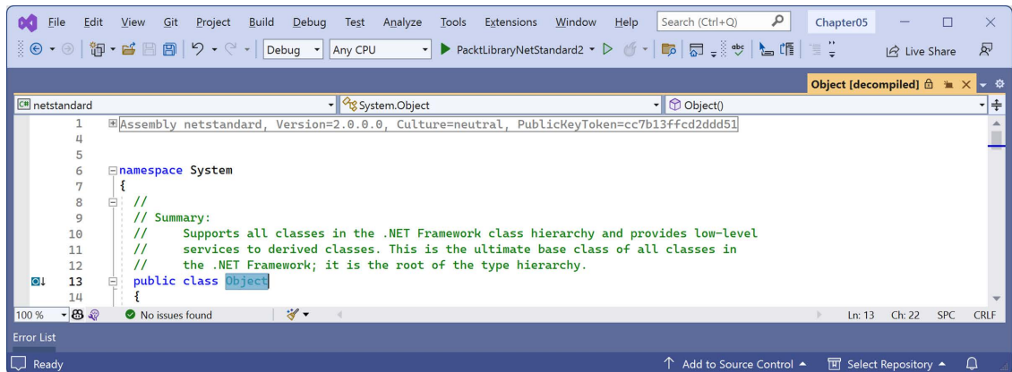
Figure 5.1: The System.Object class definition in .NET Standard 2.0
