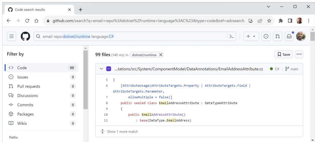
Figure 1.14: Advanced search for email in the dotnet/runtime repository
