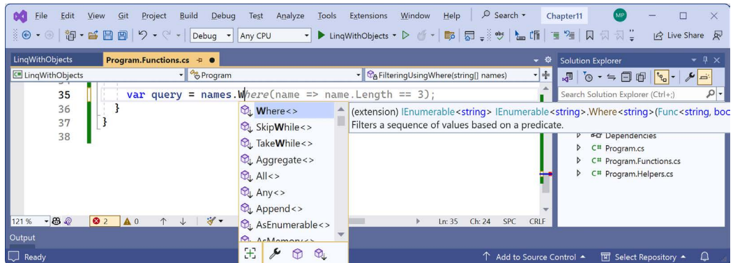
Figure 11.2: IntelliSense showing LINQ extension methods when System.Linq is imported
