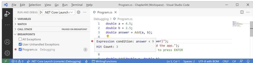
Figure 4.14: A summary of a customized breakpoint in VS Code
