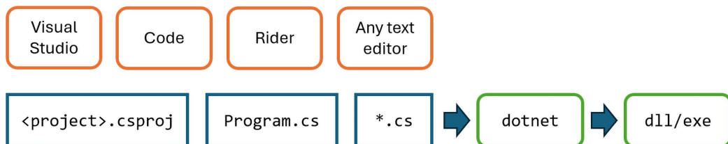
Figure 1.2: All code editors ultimately just change underlying files
