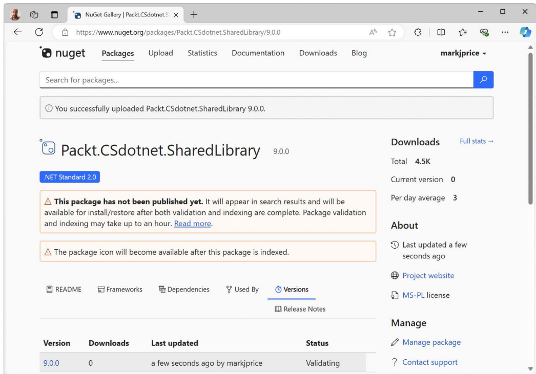
Figure 7.4: A NuGet package upload message
