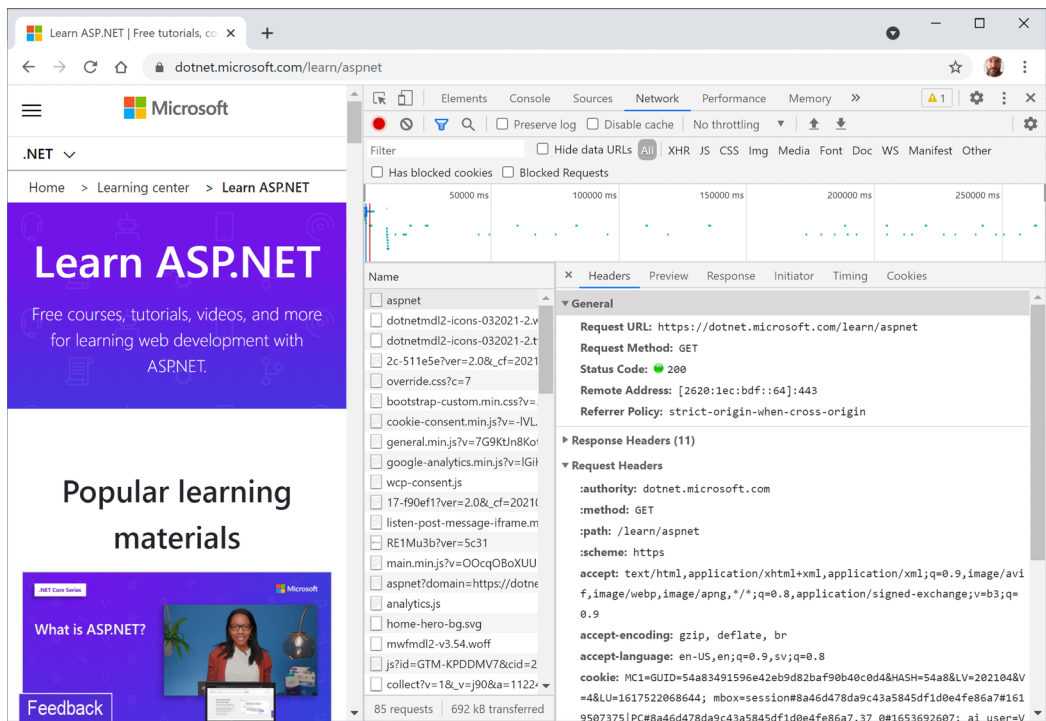
Figure 12.8: Request and response headers
