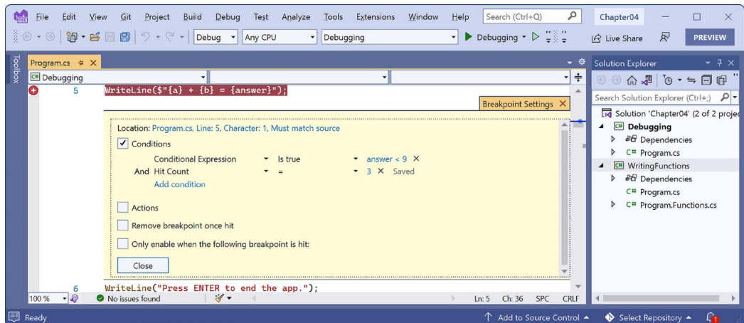
Figure 4.13: Customizing a breakpoint with an expression and hit count using Visual Studio
