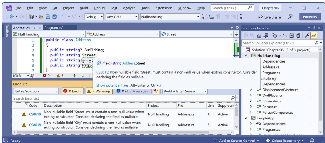
Figure 6.2: Warning messages about non-nullable fields in the Error List window
