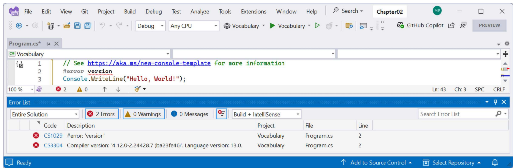
Figure 2.1: A compiler error that shows the C# language version
