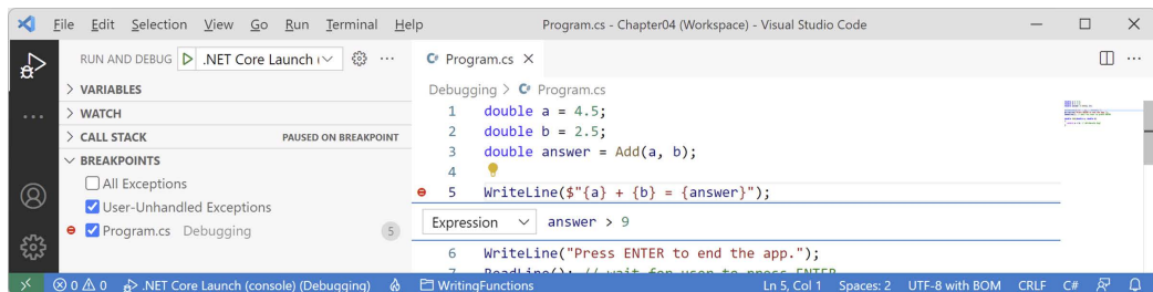
Figure 4.12: Customizing a breakpoint with an expression using VS Code
